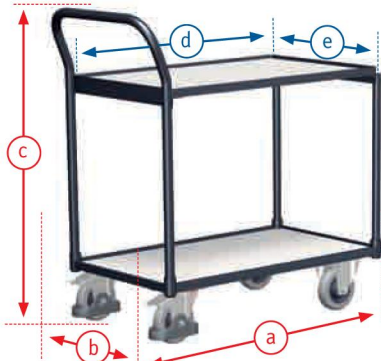
ESD table trolley Article no. esw500.557
