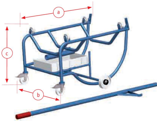
Drum dispenser Article no. ezu3201
